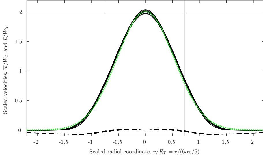
FIGURE 2. The time-averaged scaled velocities of the three plumes at 80 different heights, spanning 75 \leq z/r_0 \leq 125 , plotted against the scaled radial coordinate: vertical (solid black lines) and radial (dashed black lines) velocities. The velocities and coordinate are scaled by the predicted top-hat velocity scale W_T = (5/6\alpha)(9\alpha/10)^{1/3} F^{1/3} z^{-1/3} and top-hat radius R_T = 6\alpha z/5 , respectively, with \alpha = 0.11 . The good collapse of the data indicates that the flow exhibits the behaviour of a turbulent pure-plume and that the value of \alpha and the location of the virtual origin are correct to suitable accuracy. A best-fit normalised Gaussian distribution (dotted green line) exhibits a good fit to the vertical velocity data. A horizontal line marks \bar{w} = 2W_T , the relationship expected between the top-hat velocity and the centreline velocity assuming a Gaussian distribution. Vertical lines mark the e-folding width \tilde{R}_w which shows a close agreement to the expected relationship \sqrt{2}\tilde{R}_w = R_T .
