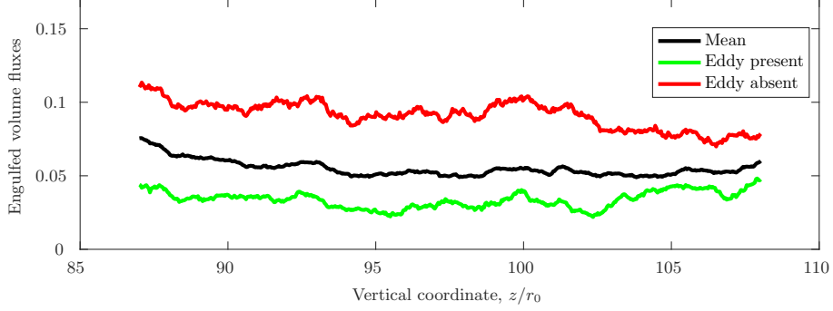
FIGURE 12. The proportion of the vertical transport which occurs as engulfed (unmixed) fluid within the plume envelope for each of the three states: mean \overline{Q_{eng}}/\overline{Q} , eddy present \overline{Q_{(eng,e)}}/\overline{Q_e} and absent \overline{Q_{(eng,n)}}/\overline{Q_n} .
