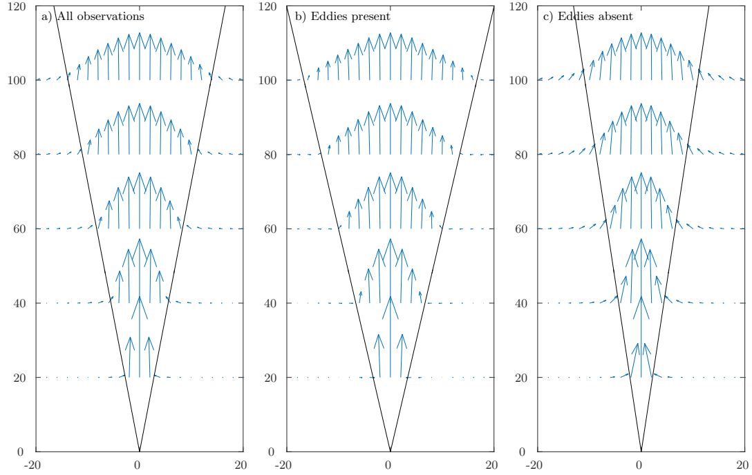
FIGURE 16. Time-averaged views of a turbulent plume: a) all observations, b) observations when eddies are present, c) when eddies are absent. The black lines mark the time-averaged position of the edge of the plume scalar field in each of the three states. The (blue) arrows mark the magnitude and direction of the measured velocity vectors (ensemble averaged over the 18 heights shown in figure 13). The axis are marked in arbitrary units.
