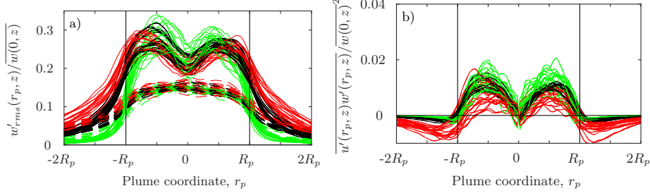
FIGURE 14. a) The root mean square of the fluctuations in vertical (solid lines) and horizontal (dashed lines) velocities and b) u'_p(z)w'_p(z)/w_p(z)|_{r_p=0}^2 averaged in the plume coordinate system, r_p . The vertical velocity fluctuations exhibit bi-modal peaks of approximately 25%–30% of the mean velocities at r_p \approx \{-0.5R_p, 0.5R_p\} . The horizontal velocity fluctuations exhibit a broad peak around the centreline, the peak values are almost 15% of the mean vertical velocities — this corresponds to the fluctuations being approximately three times larger than the maximum time-averaged horizontal velocities within the plume.
