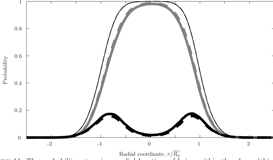
FIGURE 11. The probability, at a given radial location, of being within the plume (thin black lines), finding mixed fluid (thick grey lines) and finding engulfed fluid (thick black lines), from ensemble averages of the three plumes over all heights for which reliable data was obtained. Solid lines mark the results from the standard edge detection algorithm and dashed lines those from the alternate algorithm.
