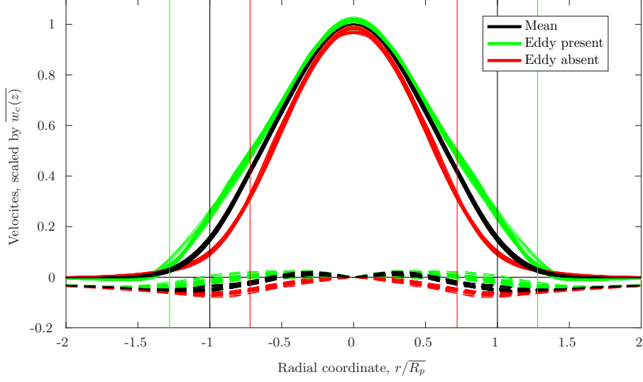
FIGURE 9. Radial distributions of vertical (solid lines) and horizontal (dashed lines) velocities, in the scaled plume coordinate. Observations of the velocities conditioned on the local presence of large-scale coherent structures are included. Vertical lines mark the time-averaged position of the plume edge in the mean (black), eddy present (green), eddy absent (red). The data show significant vertical velocities outside the plume when eddies are absent and almost no vertical flow outside the plume when eddies are present.
