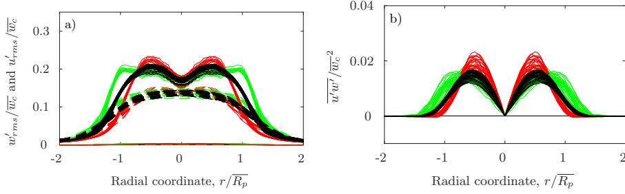
FIGURE 10. Radial distributions of a) vertical (solid lines) and horizontal (dashed lines) velocity fluctuations and b) Reynolds stresses, in the scaled plume coordinate. Observations conditioned on the local presence of large-scale coherent structures are included. The data show Reynolds stresses of slightly greater magnitude when coherent structures are absent.
