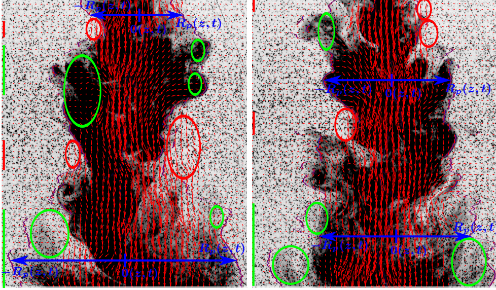
FIGURE 1. Two typical experimental images of a plume. The small dark ‘spots’ in both images are the 50\,\mu\text{m} particles used to obtain PIV measurements. Dense ‘plume fluid’, stained by dye, is indicated by dark regions in each image. The edges detected by both algorithms are marked by the red solid lines (7 pixels wide) and blue solid lines (3 pixels wide). Velocity vectors (red arrows) indicate the local two-dimensional velocity on the vertical central plane of the plume. Notice that where large-scale eddies are locally present the vertical velocities are small just outside and inside the plume edge (circled in green). At the locations where eddies are locally absent the vertical velocities outside the plume are significant (circled in red). The heights at which the measurement of the local width R_p indicate that large-scale coherent structures are present and absent are indicated by coloured bars (green present, red absent) on the left-hand edges of the two images.
