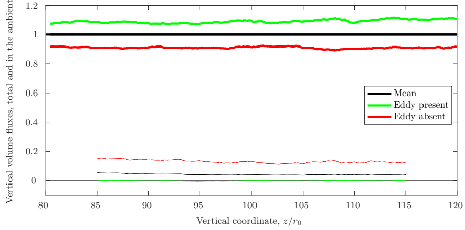
FIGURE 8. The dimensionless volume fluxes (thick lines) when eddies are present (green) and absent (red) relative to the mean, i.e. \overline{Q_e}/\overline{Q} and \overline{Q_n}/\overline{Q} , respectively. The proportion of the vertical transport occurring outside the plume are also shown for each of the three states, i.e. mean \overline{Q_{out}}/\overline{Q} (thin black lines), eddy present \overline{Q_{(out,e)}}/\overline{Q_e} (thin green lines) and absent \overline{Q_{(out,n)}}/\overline{Q_n} (thin red lines).
