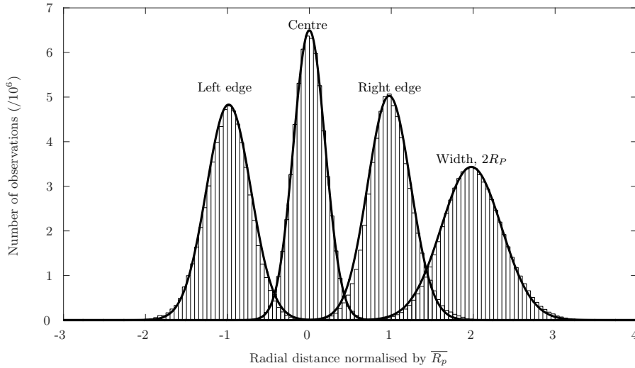
FIGURE 5. Histograms of the location of the centre, left- and right-hand edge of the plume scalar field and the magnitude of the width of the plume scalar field. All distances have been normalised by the time-average of the local half-width of the scalar edges of the plume, \bar{R}_p . The histograms contain observations from each of the three plumes, from both edge detection algorithms and at all heights for which reliable data was obtained — in excess of 6 \times 10^7 observations of each statistic. The best-fit Gaussian distribution is overlaid on each histogram.
