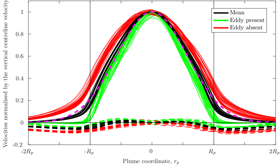
FIGURE 13. Vertical (solid lines) and horizontal (dashed lines) velocities averaged in the plume coordinate system, r_p . The full time-averaged velocities, \overline{w_p} and \overline{u_p} , are marked in black; average velocities when eddies are present, \overline{w_{(p,e)}} and \overline{u_{(p,e)}} , are marked in green; average velocities when no eddies are present, \overline{w_{(p,n)}} and \overline{u_{(p,n)}} , are marked in red. The data from three different plumes at 18 different heights exhibit a broad collapse indicating self-similarity. The vertical velocities outside the plume are significant near the plume edge and are, indeed, greater than the horizontal velocities at the same location. The dashed magenta curve is a Gaussian of variance equal to mean variance of the ensemble data (black curves).
