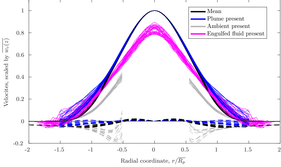
FIGURE 6. The radial distributions of vertical (solid lines) and horizontal (dashed lines) velocities, in the scaled Eulerian plume coordinate. The velocities are conditioned on the presence of plume fluid or ambient fluid, plotted at radial locations where the probability of observation exceeded 3%. The data show that fluid inside the plume moves vertically faster (by 0.1 - 0.2\bar{w}_c ) than ambient fluid at the same vertical location. Ambient fluid is accelerated both horizontally and vertically in the regions r/\bar{R}_p \approx \pm 0.5 - \pm 1.0 . The velocity profile observed when engulfed fluid is present shows that much of the vertical acceleration occurs as ambient fluid is engulfed, with engulfed fluid travelling at approximately 80% of the velocity of plume fluid locally.
