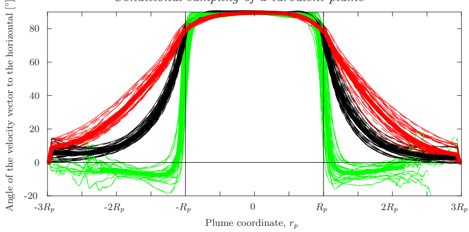
FIGURE 15. The angle to the horizontal of the velocity vectors averaged in the plume coordinate system, r_p . The angles from the full time-averages are marked in black, those averaged only when eddies are present are marked in green, and those when no eddies are present are marked in red. Steep radial gradients in the angles are only observed at the plume edge when eddies are present.
