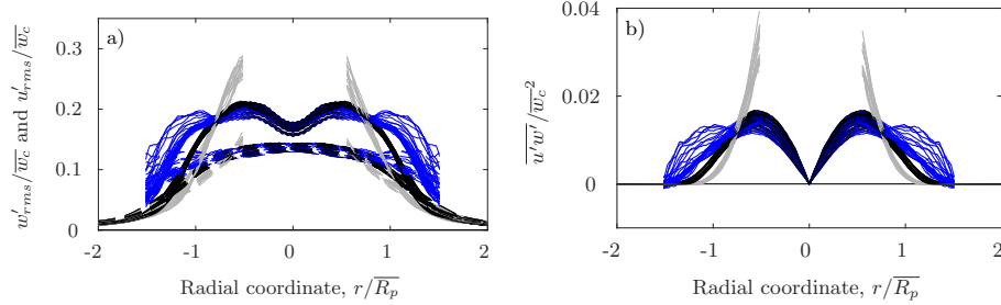
FIGURE 7. The radial distributions of a) vertical (solid lines) and horizontal (dashed lines) velocity fluctuations and b) Reynolds stresses, in the Eulerian plume coordinate. Observations are conditioned on presence of the plume or the ambient (colour scheme as in figure 6). The data show large Reynolds stresses in ambient fluid when in the regions r/\bar{R}_p \approx \pm 0.5 - \pm 0.8 .
